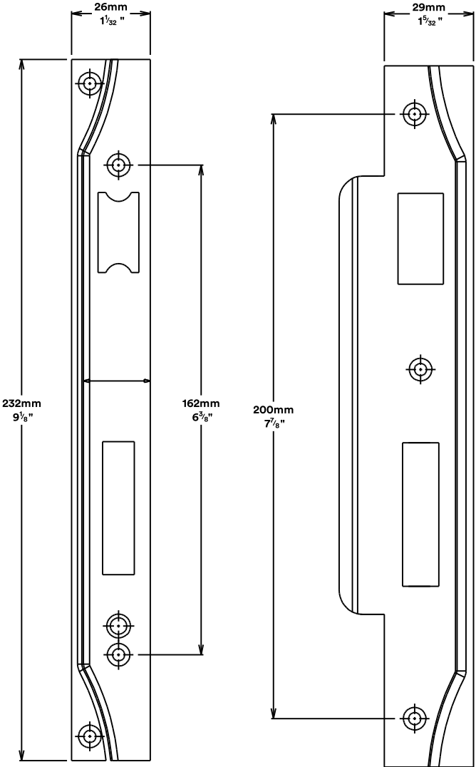
Mortice Lock & Rebated Face plate
