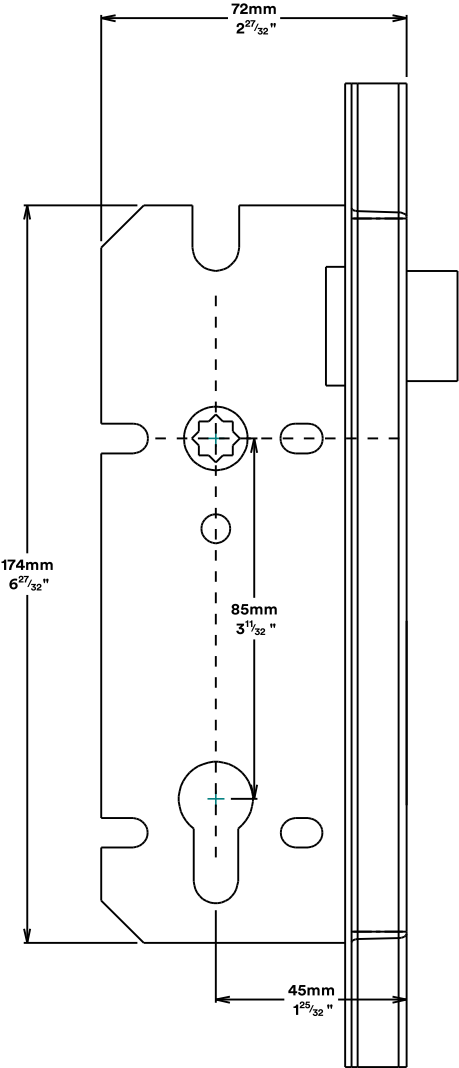
Mortice Lock & Rebated Face plate
